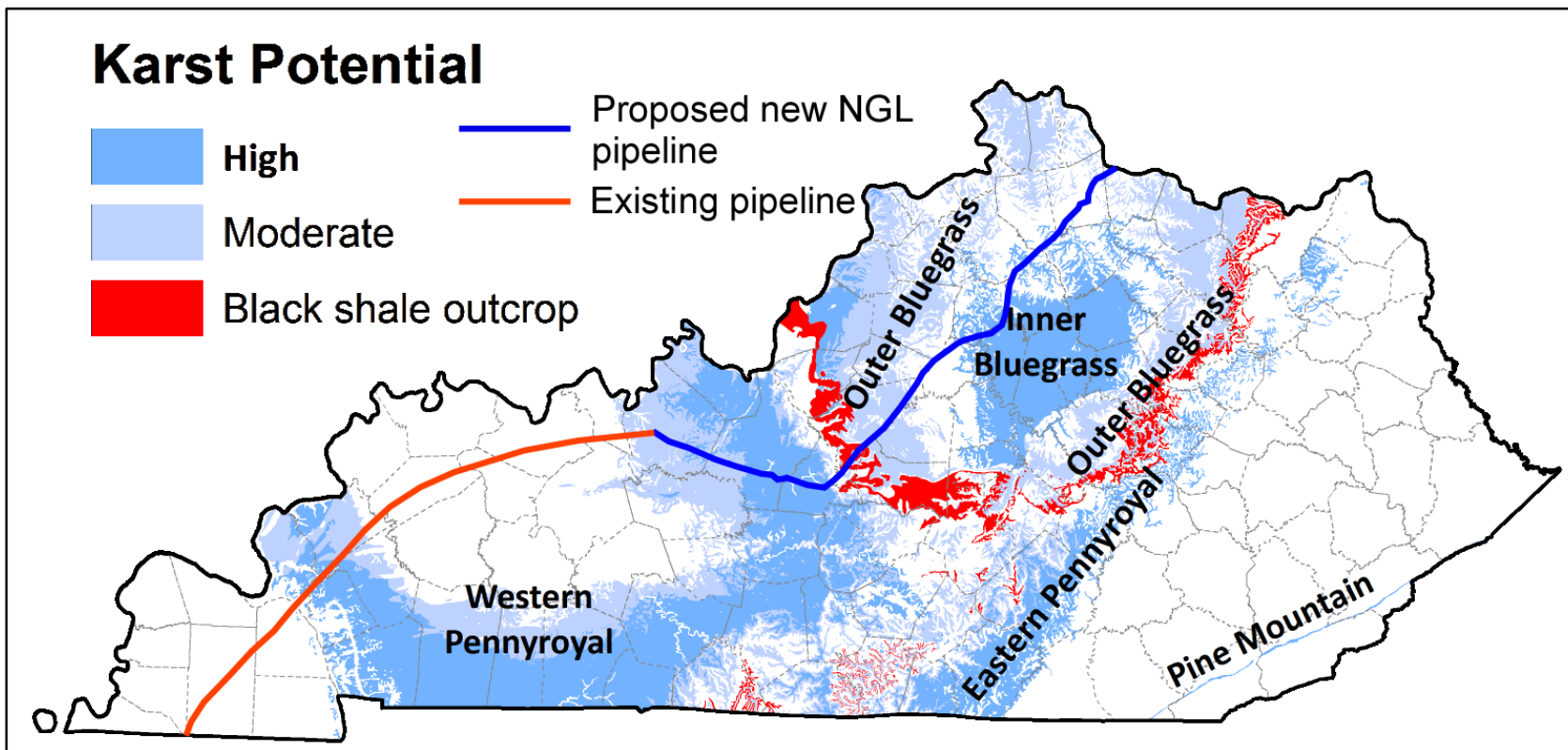
Figure 3. Generalized karst potential, karst regions, and black shale outcrop areas in Kentucky. Proposed route of new pipeline and existing natural gas pipeline to be converted are shown.
