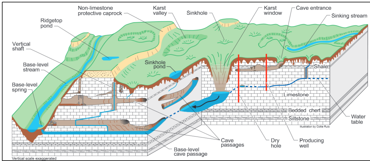
Figure 2. Karst features typical of the Western Pennyroyal area. For more information, or to view and print the generalized karst block diagrams, please visit www.uky.edu/KGS/water/general/karst/karstgis.htm .
